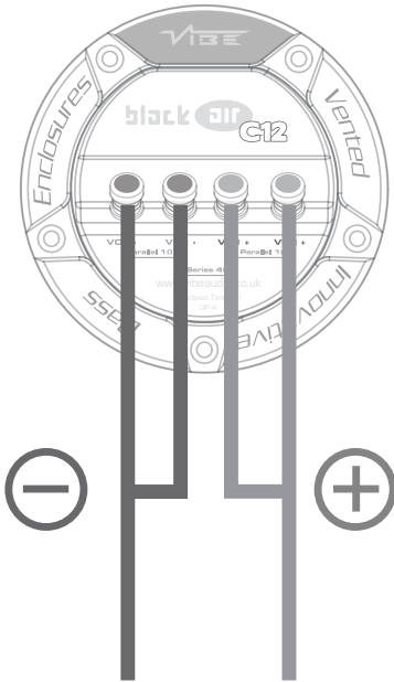
Parallel 1Ω
