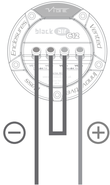
Series 4Ω
